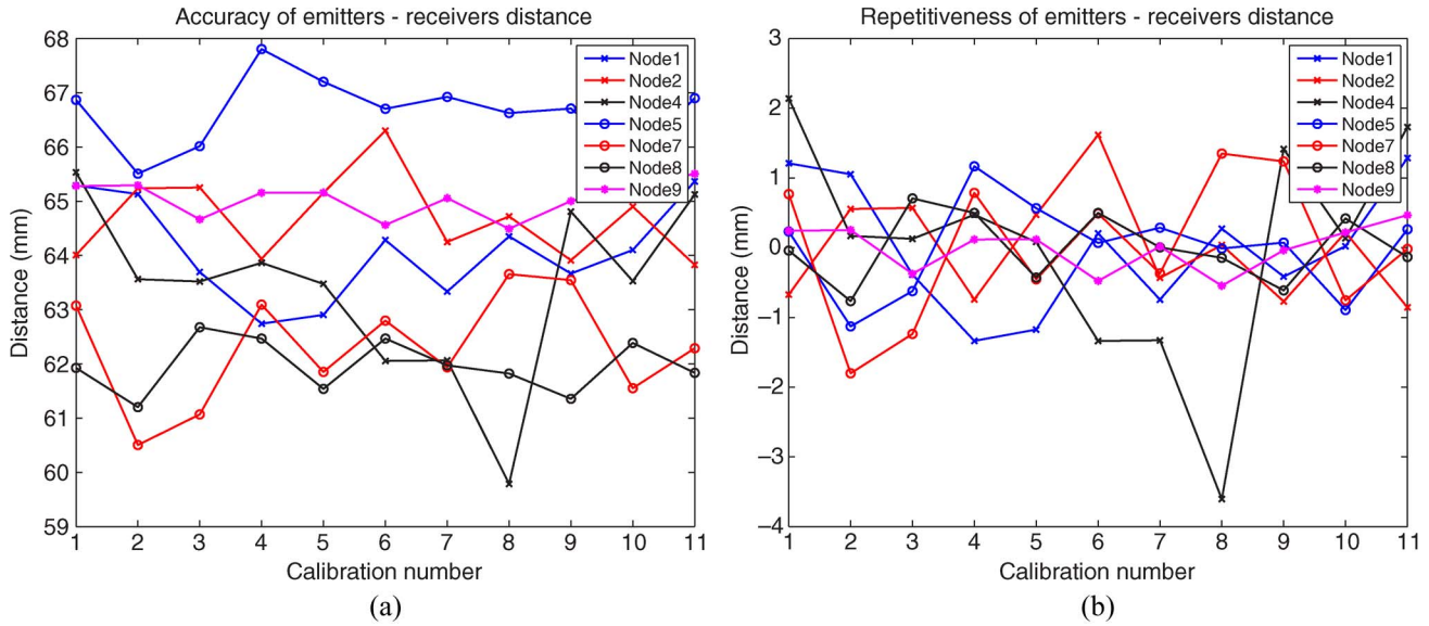
Fig. 5. Evaluation of the transducers' distance consistency of the seven fixed downward nodes for each of the 11 calibrations, showing the variation in distance obtained for separate nodes and its variation with different calibrations. (a) Distance between nodes' transducers. (b) Distance variation around their mean.
